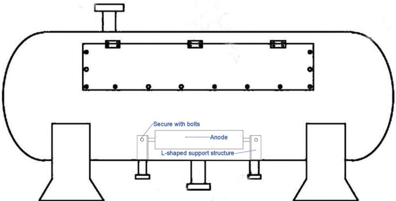
Installation Diagram
